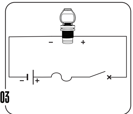
STEP 3: Using a 4A fuse, attach wires to a 12v power supply and ensure there is a waterproof connection.
