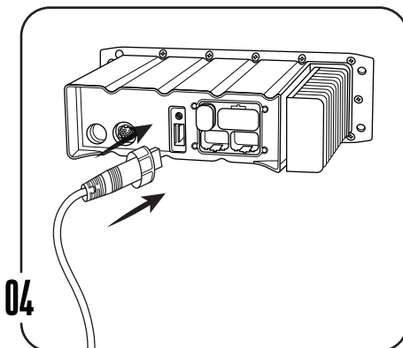
STEP 4(OPTIONAL): Connect the male USB-A 2.0 cable to onboard equipment.
